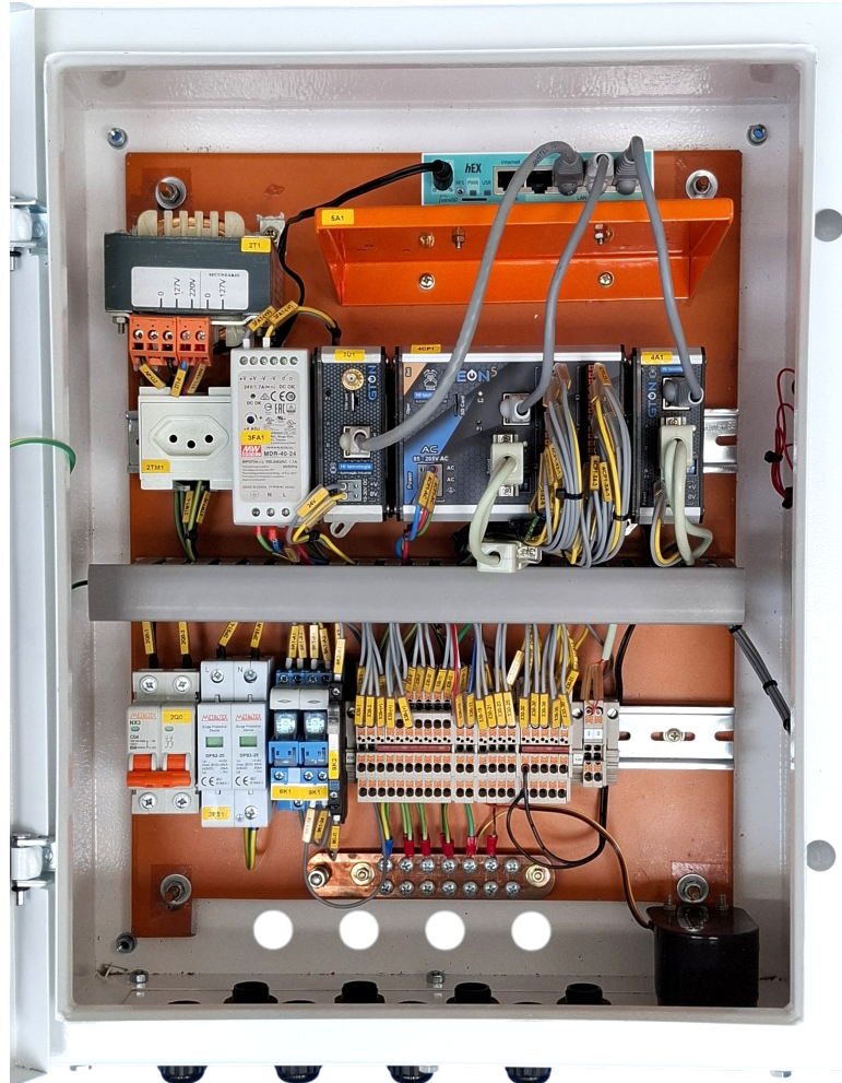
Figura 1 - Painel ACOS500 BM STD com Gateway Modbus
