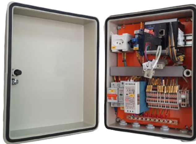
Figura 1 - Painel ACOS225 BM LT0
